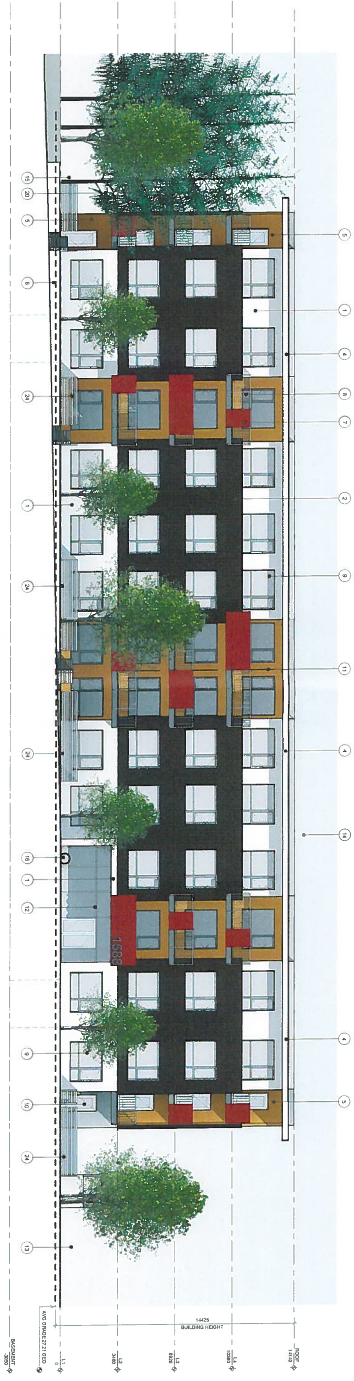
SOUTH ELEVATION
